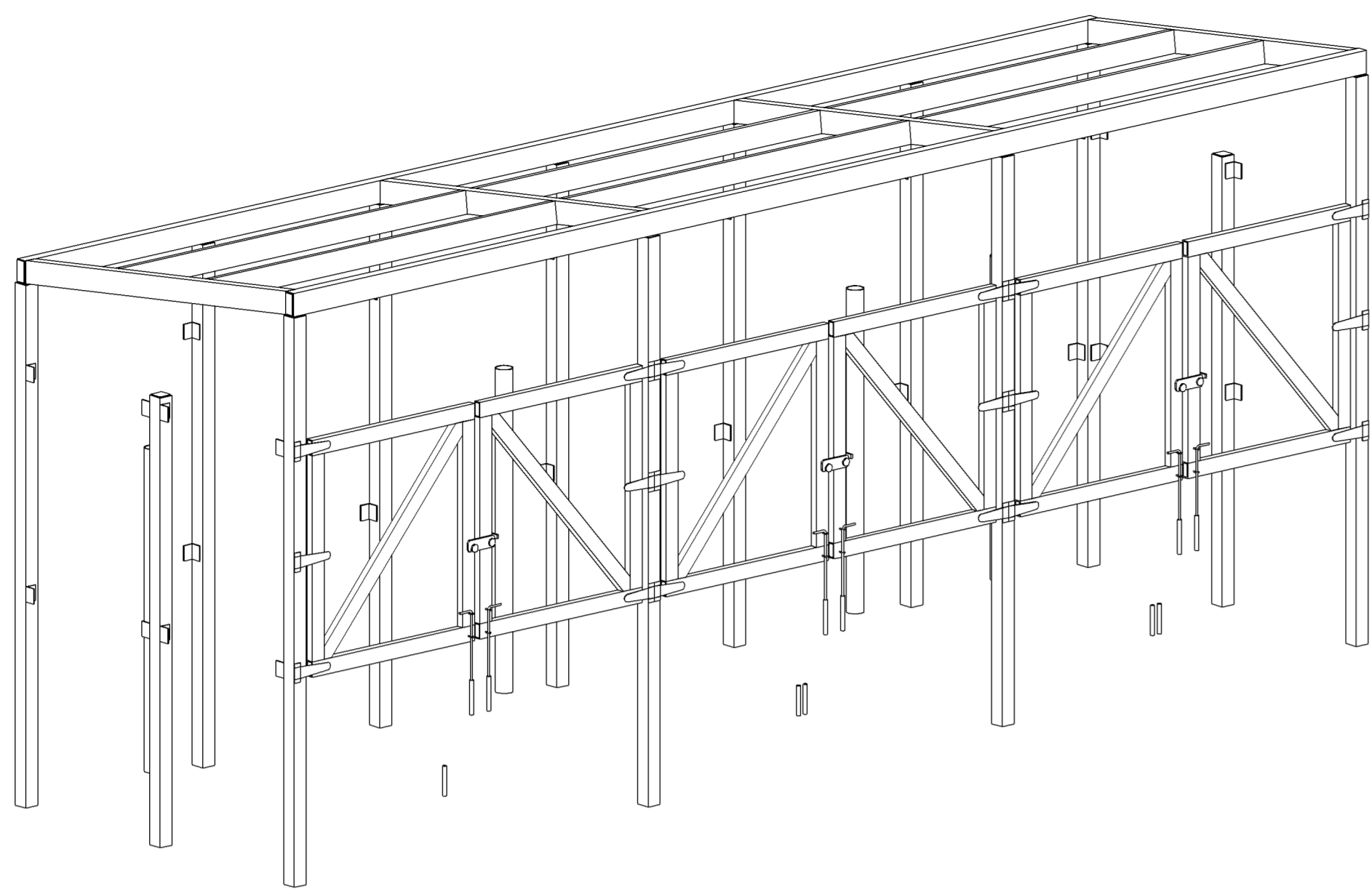
GARBAGE ENCLOSURE
