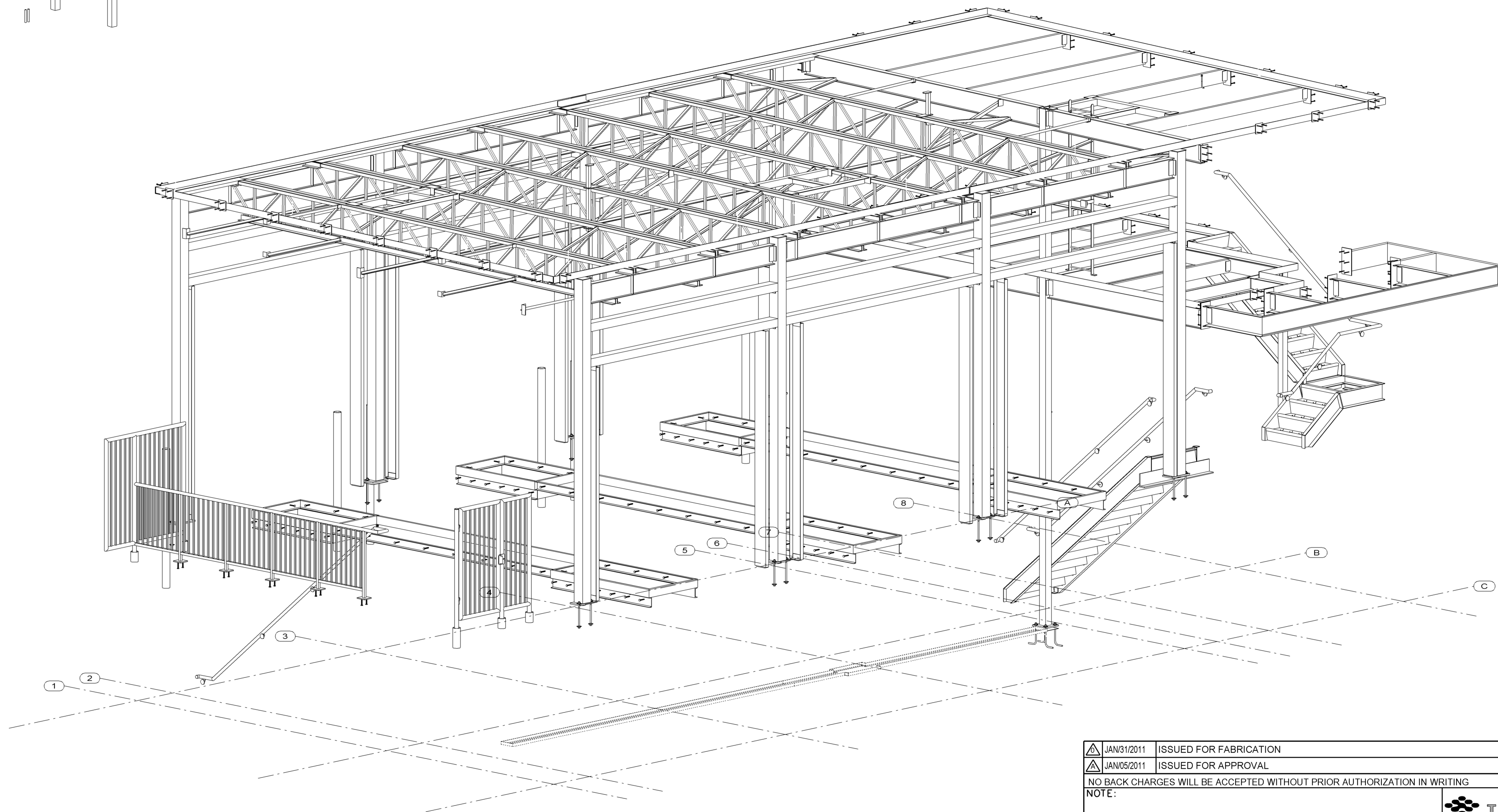
GARBAGE ENCLOSURE
